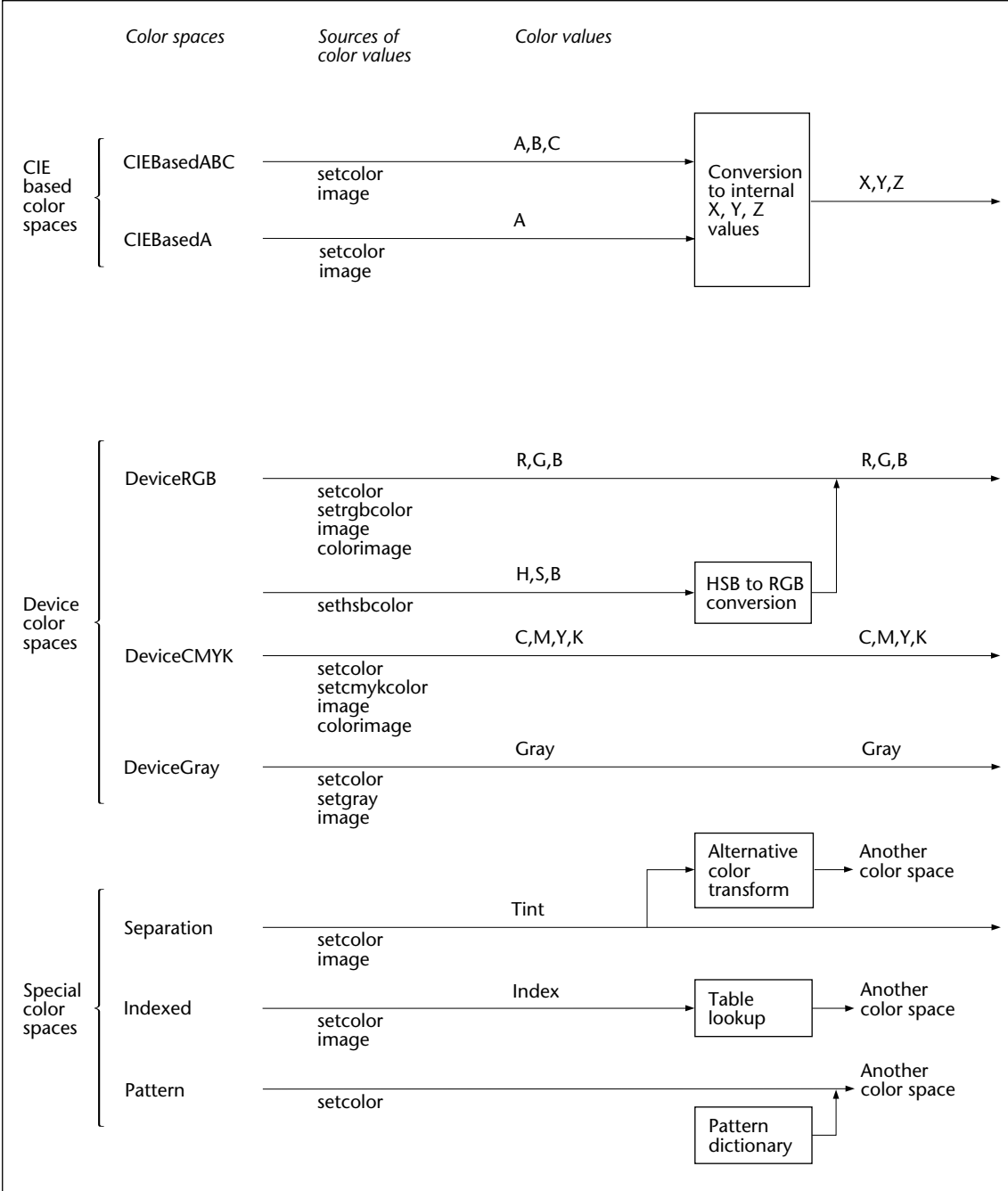
Figure 4.5 Color specification
