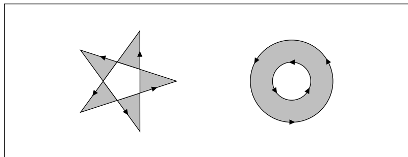
Figure 4.4 Even-odd rule
