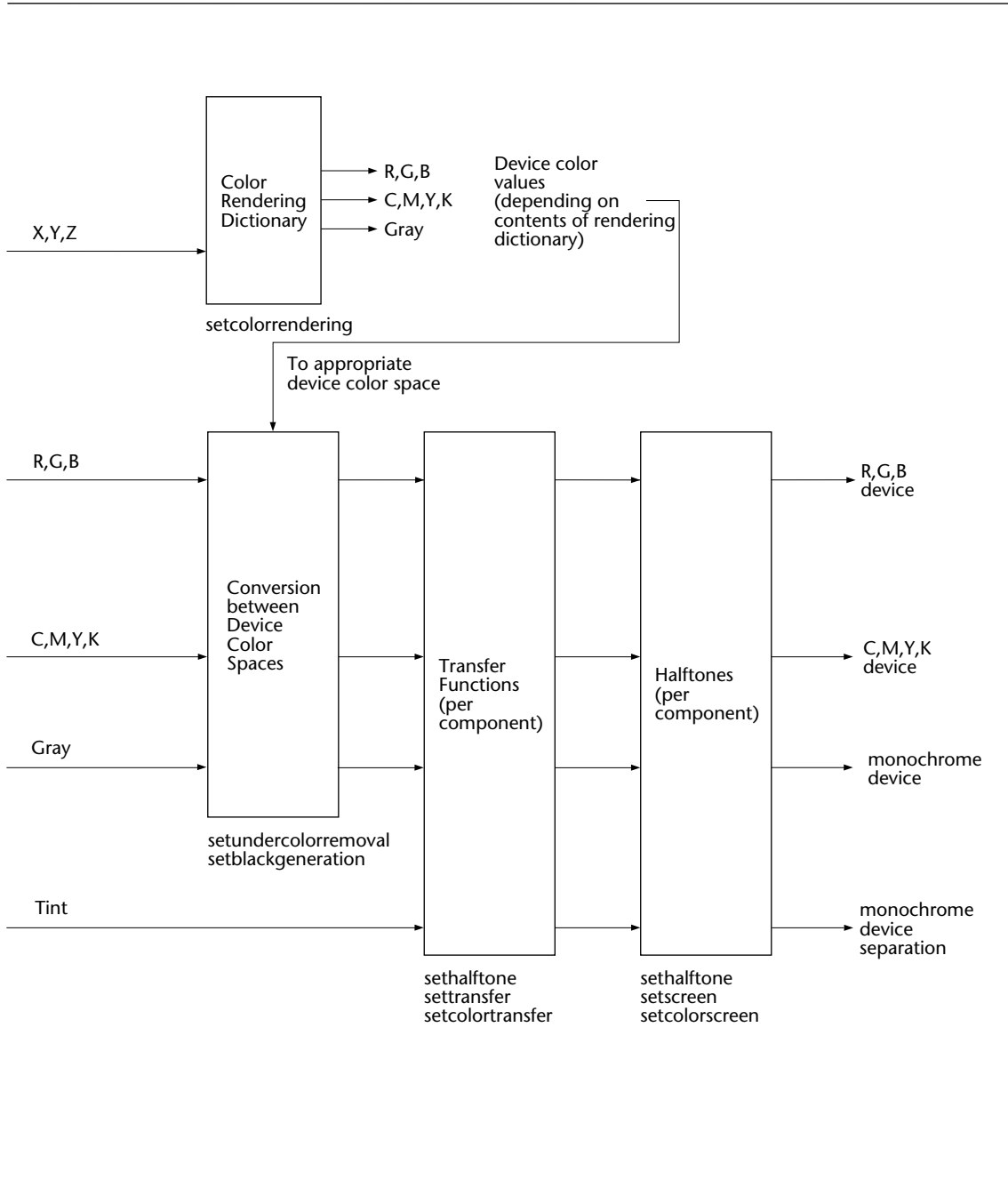
Figure 4.6 Color rendering
