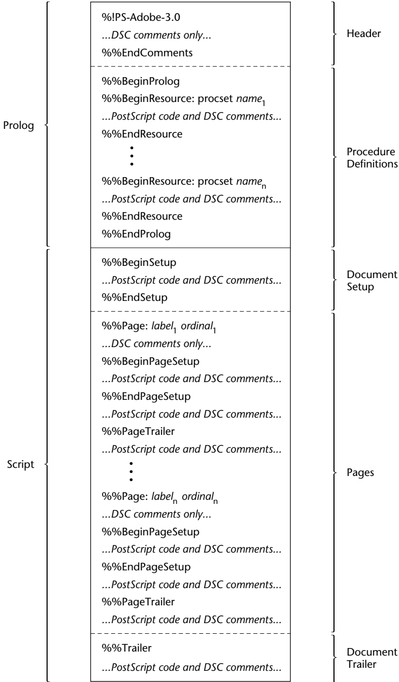
Figure G.1 Structure of a conforming PostScript language document
