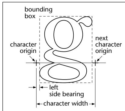
Figure 5.5 Character metrics
